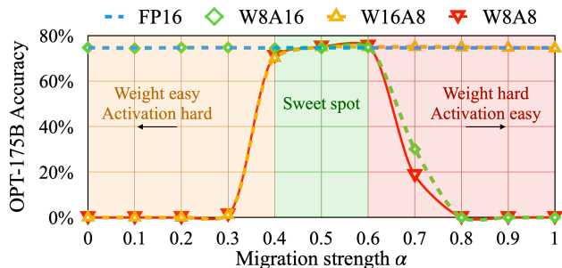
Figure 10: A suitable migration strength (sweet spot) makes both activations and weights easy to quantize. If the is too large, weights will be hard to quantize; if too small, activations will be hard to quantize.
