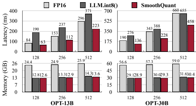
Figure 8: The PyTorch implementation of SmoothQuant-O3 achieves up to 1.51 speedup and 1.96 memory saving for OPT models on a single NVIDIA A100-80GB GPU, while LLM.int8() slows down the inference in most cases.
