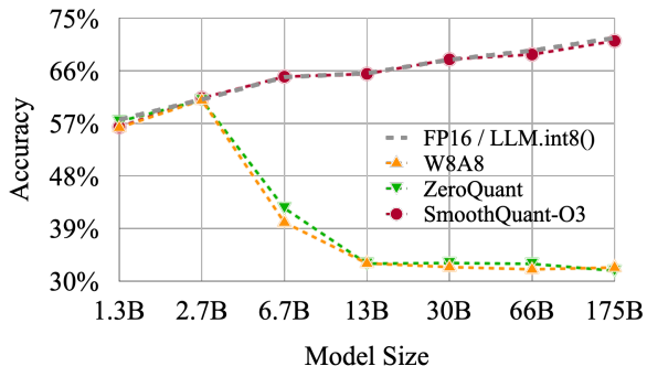
Figure 7: SmoothQuant-O3 (the most efficient setting, defined in Table 2) preserves the accuracy of OPT models across different scales when quantized to INT8. LLM.int8() requires mixed precision and suffers from slowing down.
